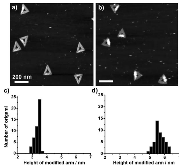
Figure 3. a,b) AFM images showing the site-specific incorporation of DNA3 and the subsequent in situ synthesis and site-specific immobilization of AgNCs on a particular arm of the triangular DNA origami scaffolds before (a) and after (b) treatment with the Tollens reagent ( z scale = 10 nm). c,d) Corresponding histograms showing the height of the bright feature on the origami before (c) and after (d) treatment with the Tollens reagent.
